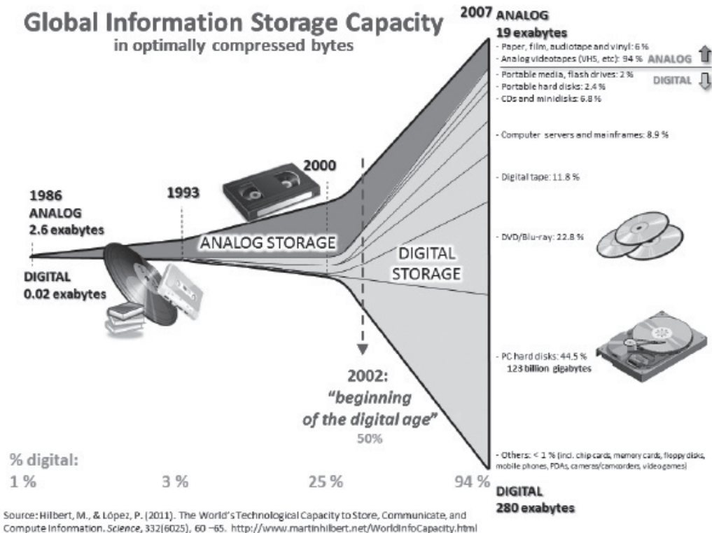
Figure 1. Global information Storage Capacity from 1986 to 2007.
