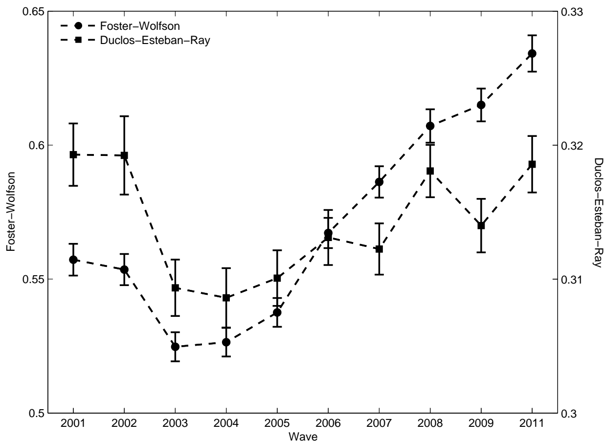
Figure 3 Polarization measures for the income distribution of Brazilian households, 2001–2011. Vertical bars represent 95% confidence intervals. The Duclos-Esteban-Ray index has been computed with the polarization sensitivity parameter \alpha set at 0.5.
