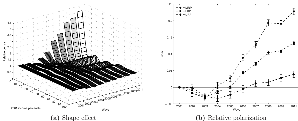
Figure 2 Trend of relative distribution in Brazil, 2001–2011. In panel (b), the 95% pointwise confidence intervals, shown by error bars, are indicated for the null hypothesis of no change with respect to the reference year, i.e. that the index equals 0
