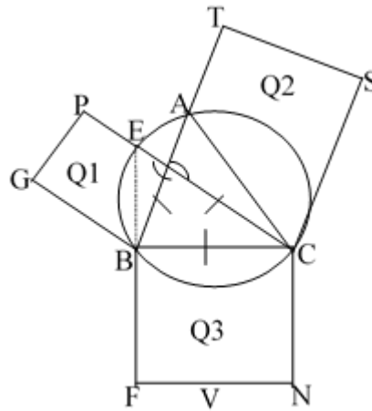
Figura 2 – Pythagoras’ Theorem
