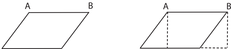
Fig. 3 Wertheimer's parallelogram problem: the area of the parallelogram can be found by transforming the parallelogram into a rectangle (as shown in the figure on the right; for further discussion, see text).
