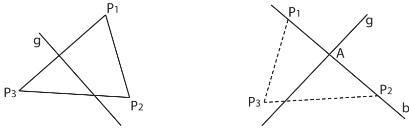
Fig. 2 The figure shows, on the left, a demonstration of Pasch's theorem and, on the right, the configuration to which it is to be applied (taken from Duncker 1945, 104).
